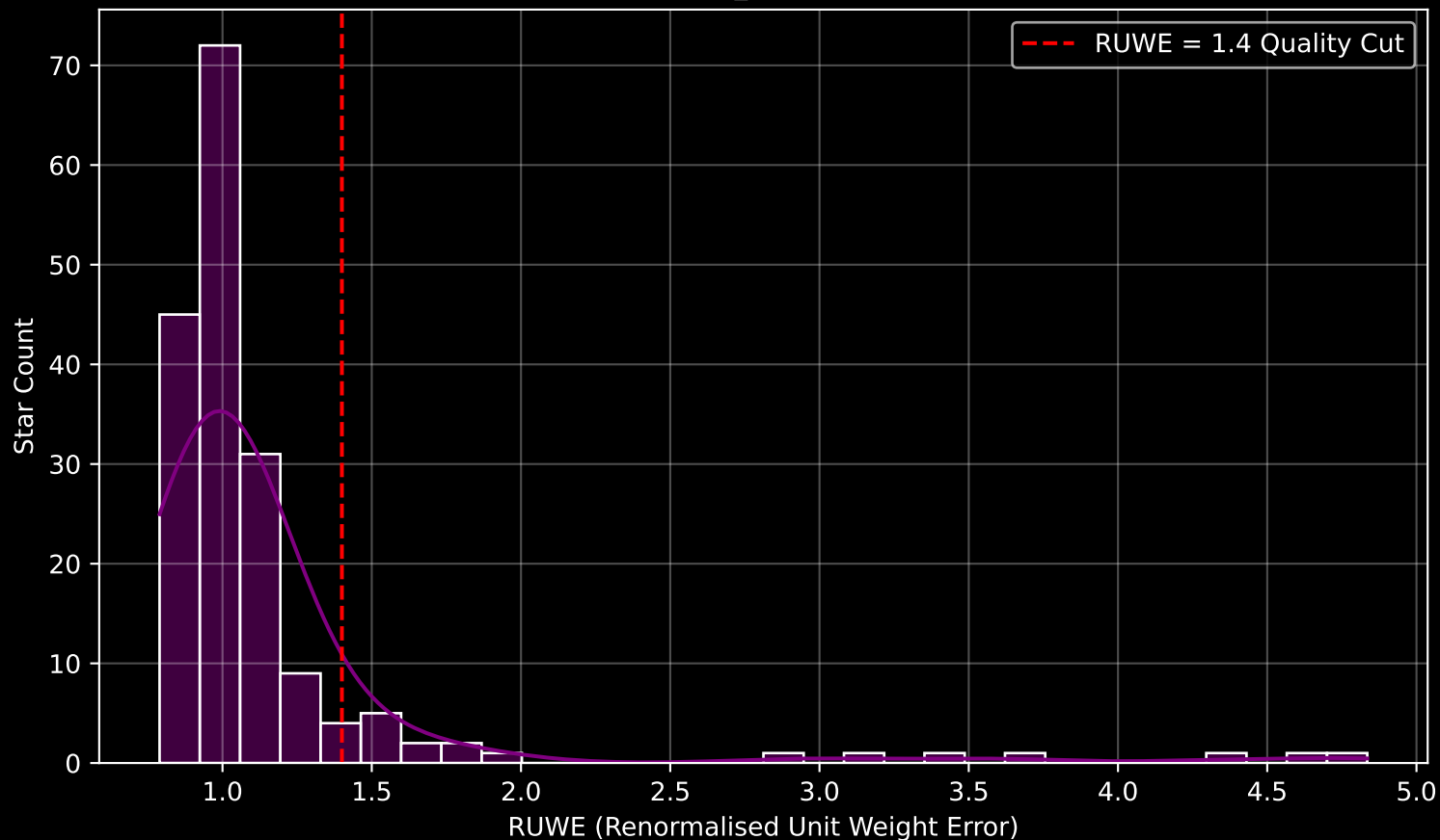
GAPOGEE DR17 Field [193+43_MGA] RUWE Distribution (n= 178)
