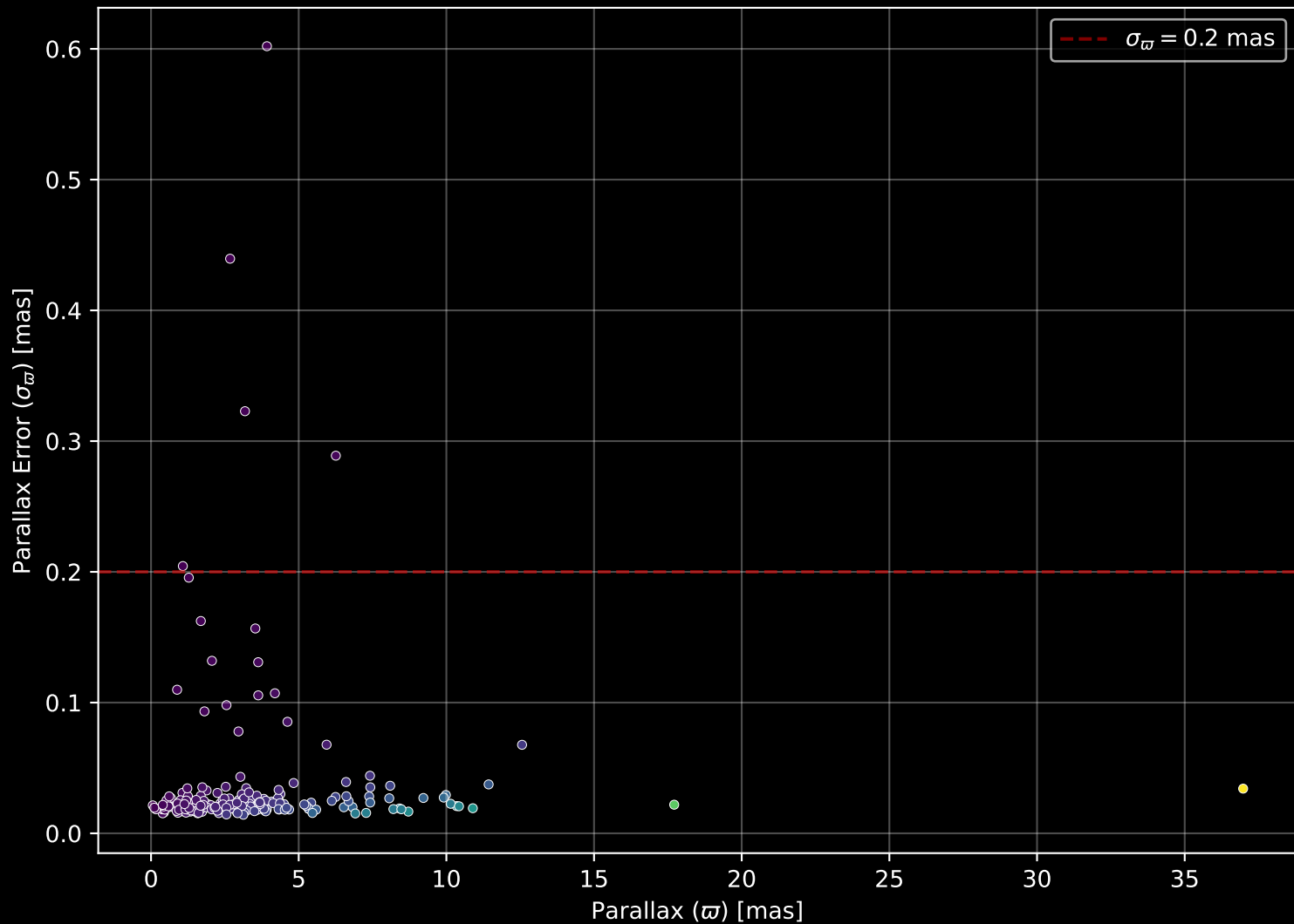
APOGEE DR17 Field: [193+43_MGA] Parallax Quality (n= 190)
