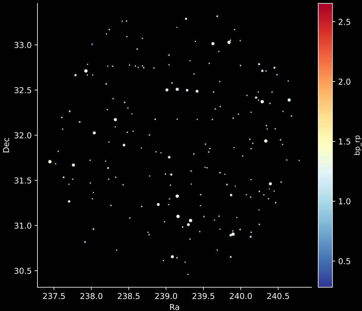
APOGEE DR17 Field: [193+43_MGA] Stars: 190
