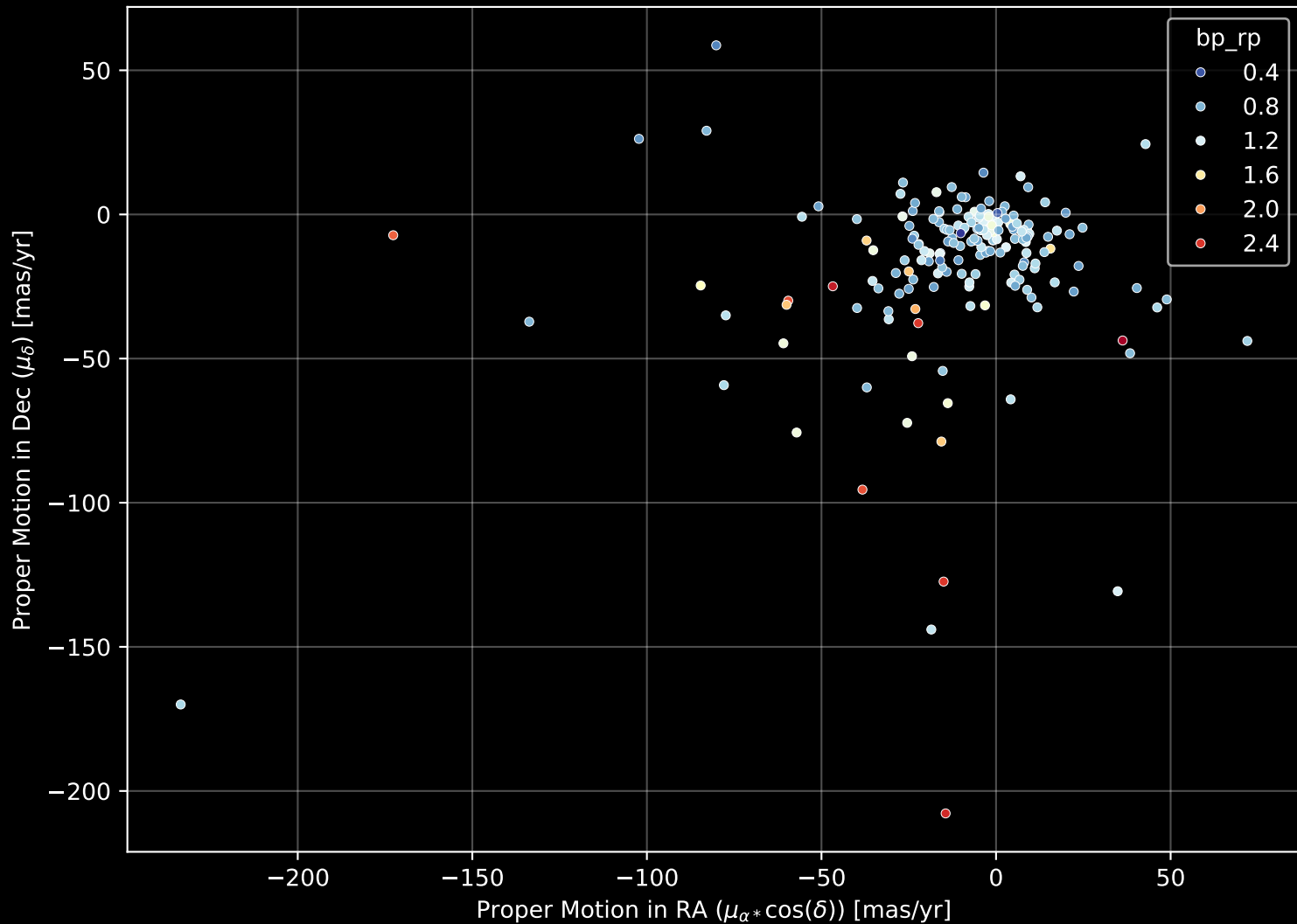
APOGEE DR17 Field: [193+43_MGA] Proper Motion Diagram (n= 190)
