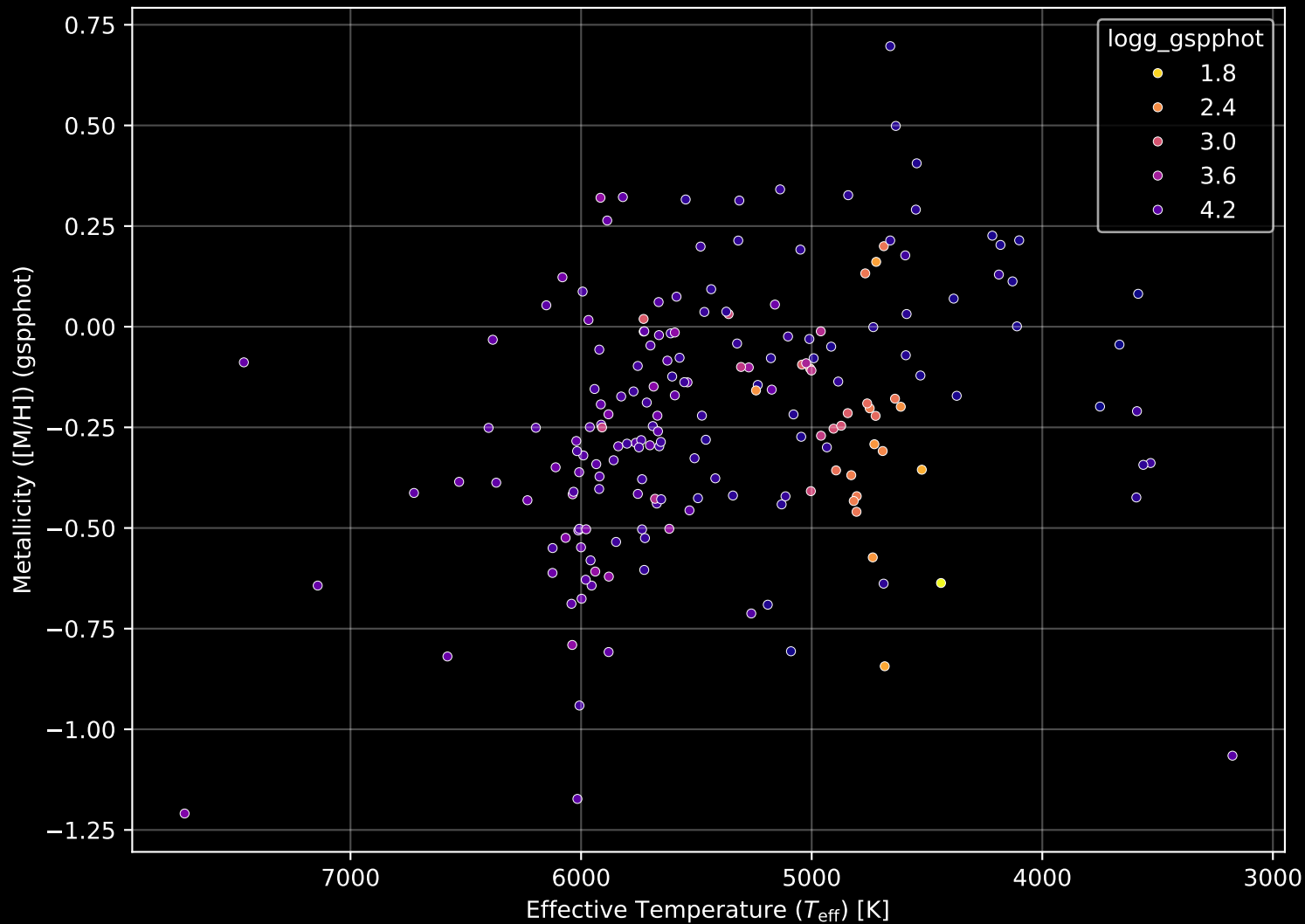
APOGEE DR17 Field: [193+43_MGA] Stellar Population Parameters (n= 190)
