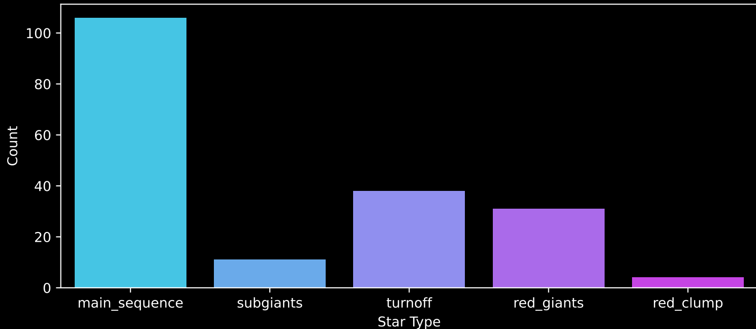
APOGEE DR17 Field: [193+43_MGA] Count plot of Star Type
