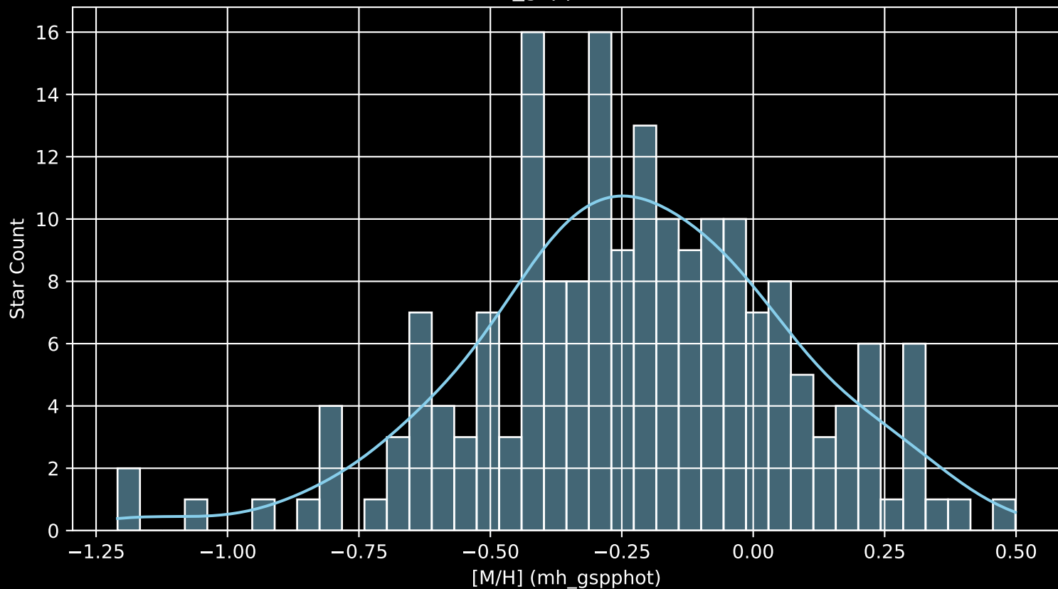
APOGEE DR17 Field: [193+43_MGA [M/H] (mh_gspphot) (n= 189)
